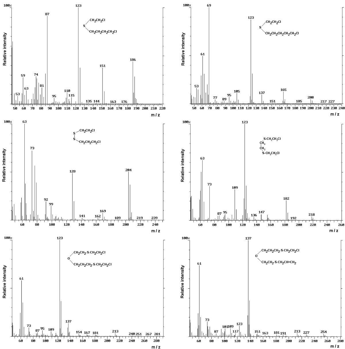
Fig. 4. The selected mass spectra of some compounds detected in the dichloromethane extract of the yperite block.
