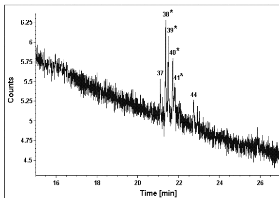
Fig. 2. Oxygen chromatogram (O–171 nm) of a sample of the yperite block obtained by GC–AED. Starlets mark oxygen mustards. The peaks of 37 and 44 represent aliphatic ethers.
