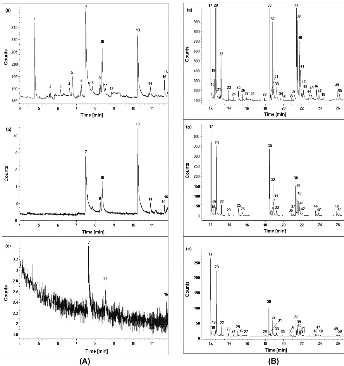
Fig. 1. (A) The first part of the element chromatograms of a sample of the yperite block obtained by GC–AED on channel: (a) carbon, C–193 nm, (b) sulphur, S–181 nm and (c) chlorine, Cl–479 nm; split ratio 20:1. (B) The second part of the element chromatograms of a sample of the yperite block obtained by GC–AED on channel: (a) carbon, C–193 nm, (b) sulphur, S–181 nm and (c) chlorine, Cl–479 nm; split ratio 60:1.
