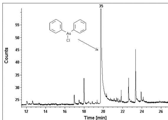
Fig. 3. Element chromatogram of chlorodiphenylarsine (Clark I) detected in the sample of the yperite block obtained by GC–AED on arsenic channel (As–189 nm). The remaining peaks originate from environmental residues.
